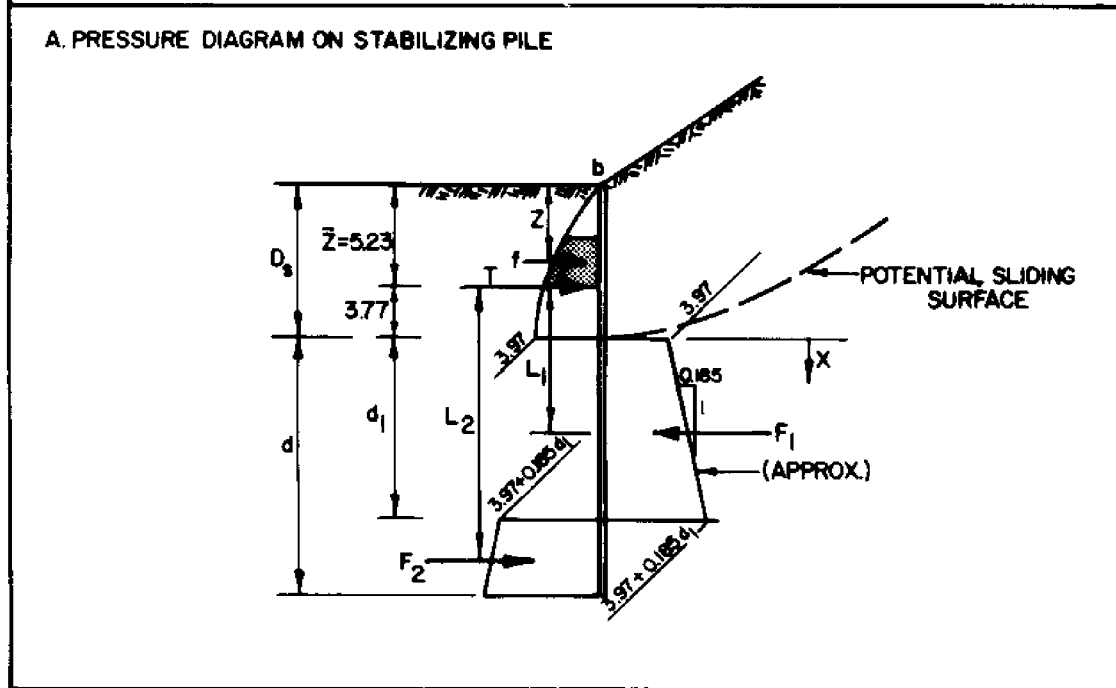
FIGURE 13 Example Calculation - Pile Stabilized Slopes
