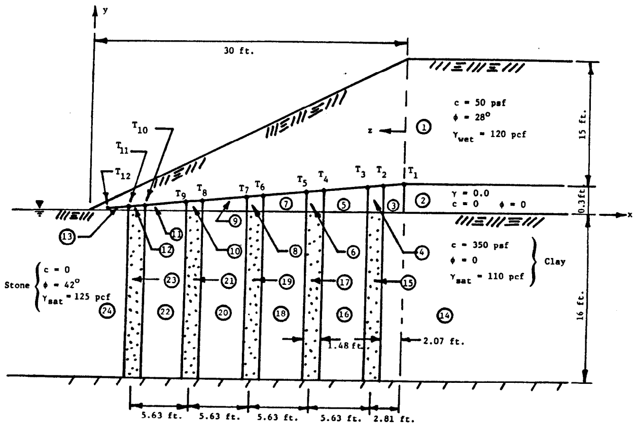
FIGURE 102. ZONES USED FOR COMPUTER IDEALIZATION FOR STABILITY EXAMPLE 1.
