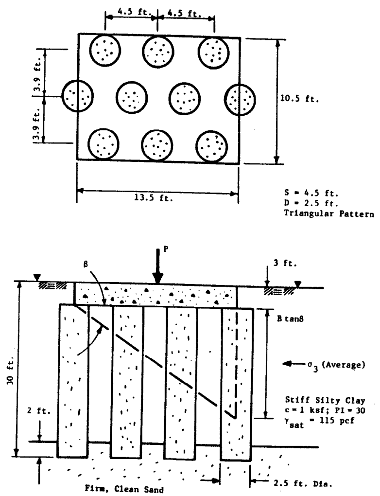
FIGURE 97. BEARING CAPACITY EXAMPLE 2.
