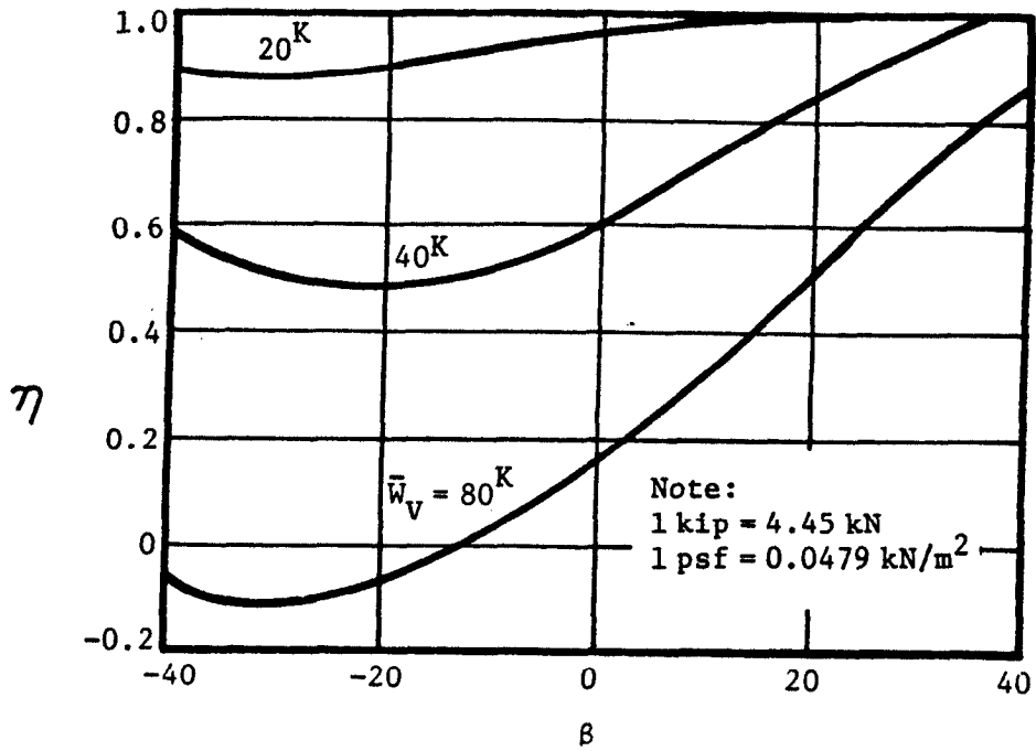
FIGURE 87. LOCAL BEARING FAILURE STABILITY REDUCTION FACTORS FOR DEEP FAILURE: \phi = 36^\circ , c = 200 PSF.
